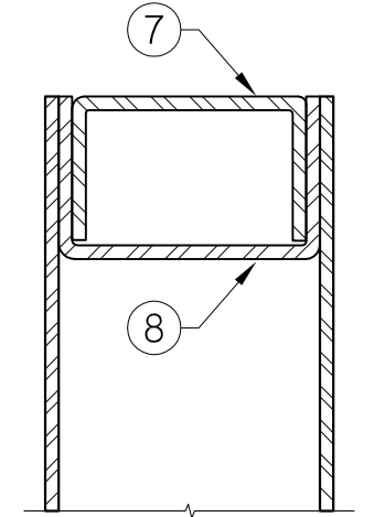
TOP/BOTTOM END CHANNELS
