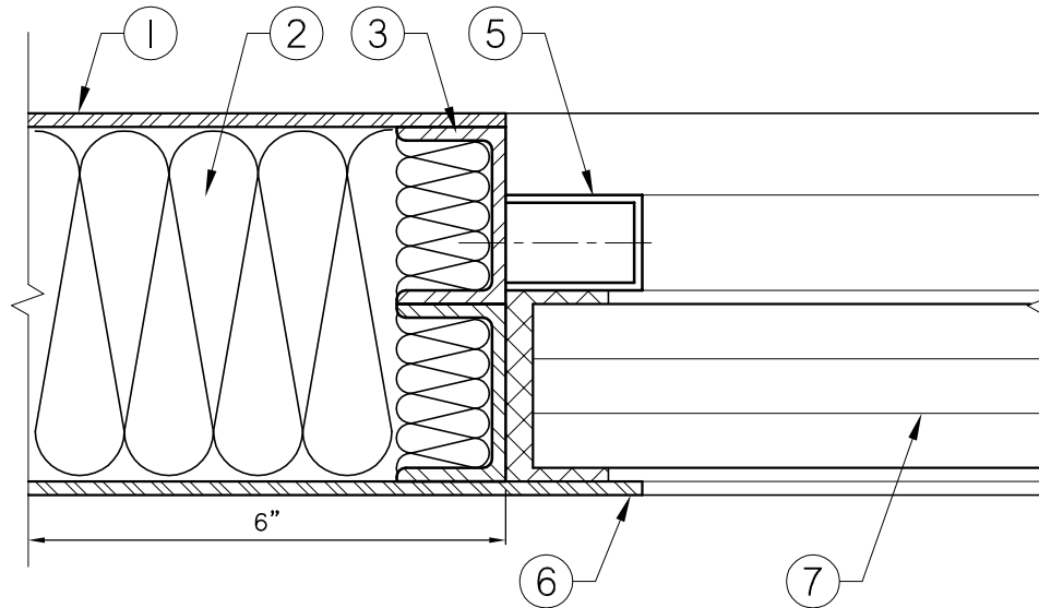
TYPICAL VISION LITE SECTION 'B'
