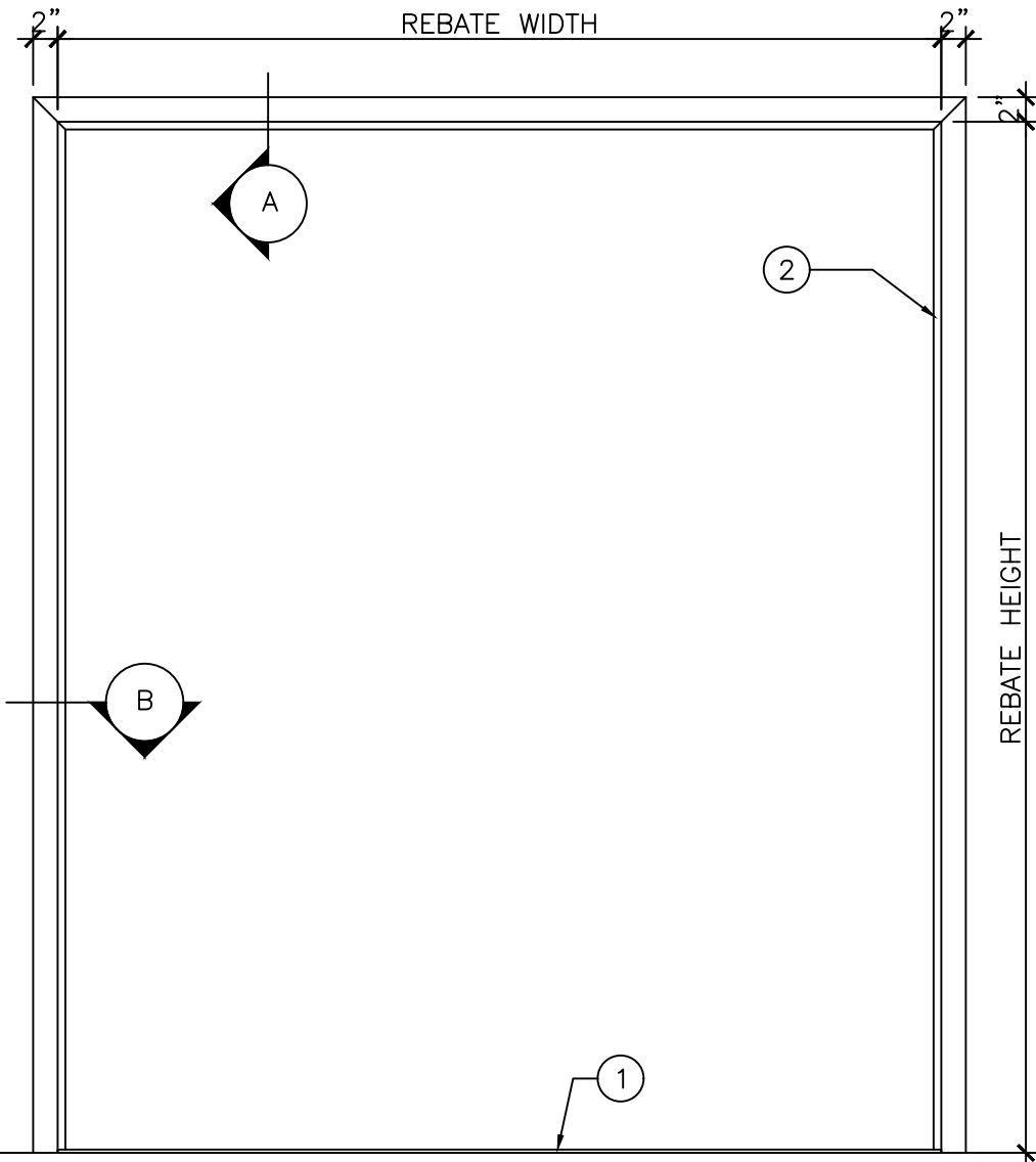
ELEVATION 3/4" = 1'-0"
