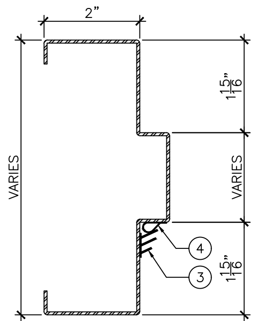
DETAIL "B" 6" = 1'-0"
