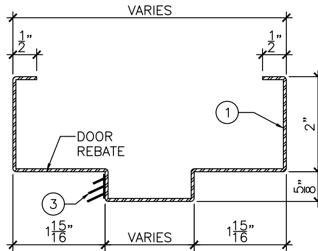
DETAIL "A" 6" = 1'-0"
