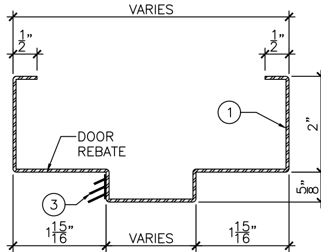
DETAIL "A" 6" = 1'-0"
