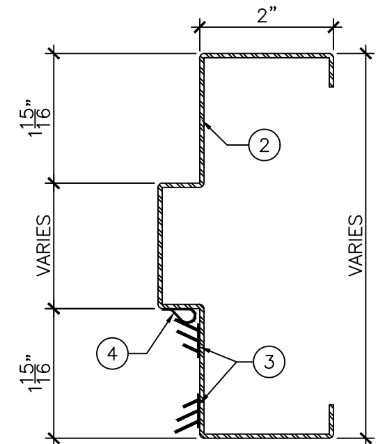
DETAIL "C" 6" = 1'-0"
