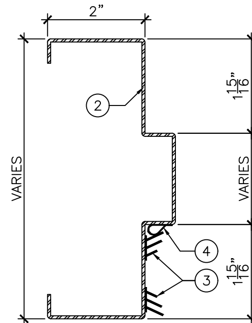
DETAIL "B" 6" = 1'-0"
