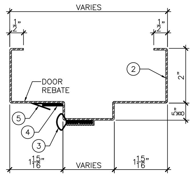
DETAIL "A" 6" = 1'-0"
