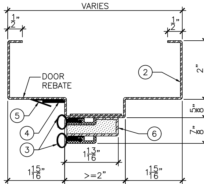
DETAIL "A" - 2" SOFFIT OR MORE 6" = 1'-0"
