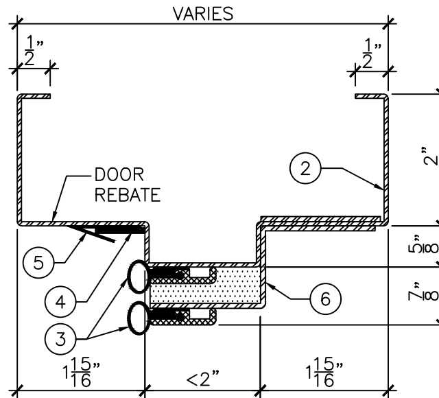
DETAIL "A" - LESS THAN 2" SOFFIT 6" = 1'-0"
