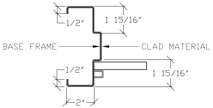
SECTION A - TYPICAL CLAD FRAME
