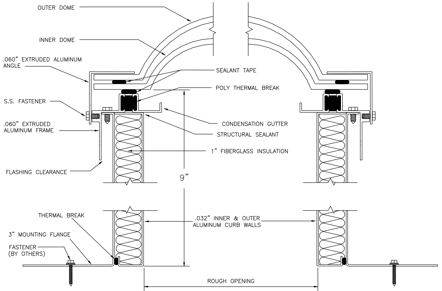
9" THERMALLY BROKEN & INSULATED SELF FLASHING (MODEL TSF-9)
