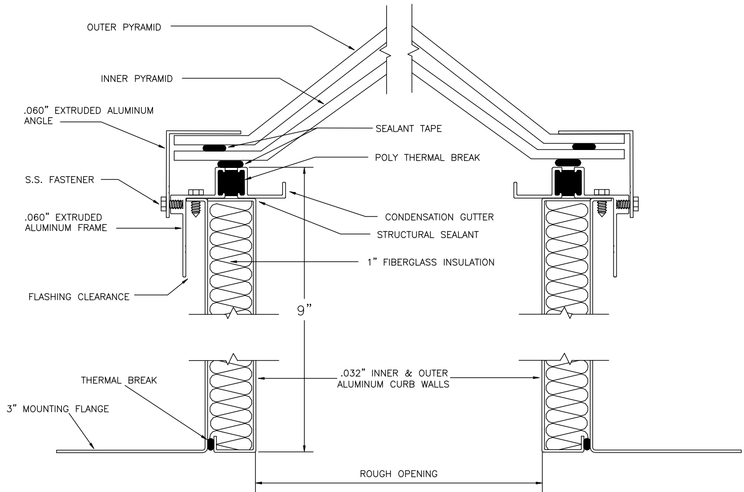
9" THERMALLY BROKEN & INSULATED SELF FLASHING – PYRAMID (MODEL TSF-9-PYR)
