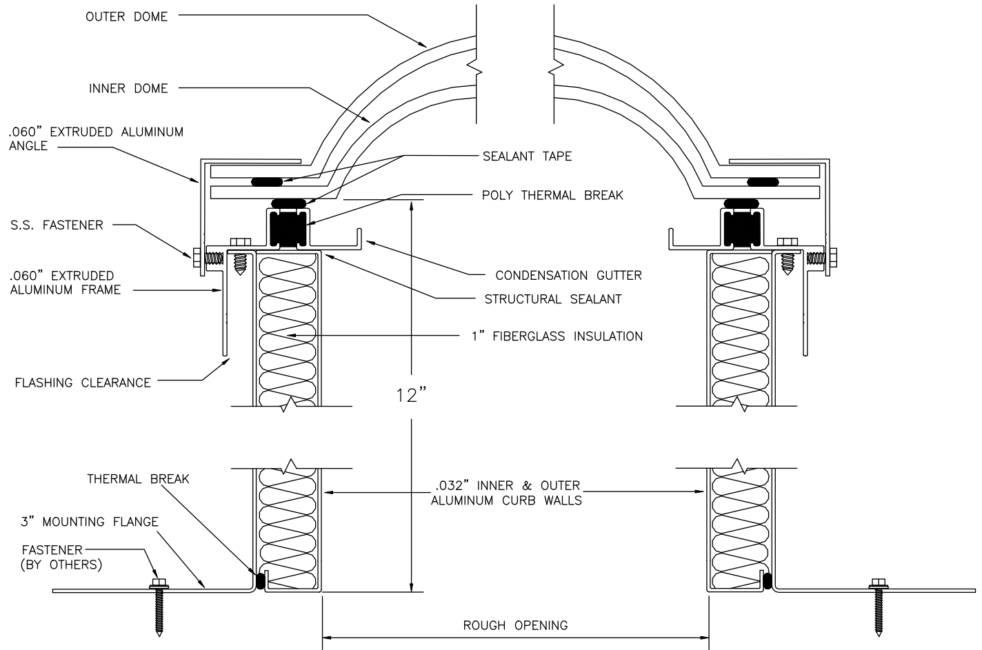
12" THERMALLY BROKEN & INSULATED SELF FLASHING FALL PROTECTION RATED UNIT (MODEL TSF-12-FG)
