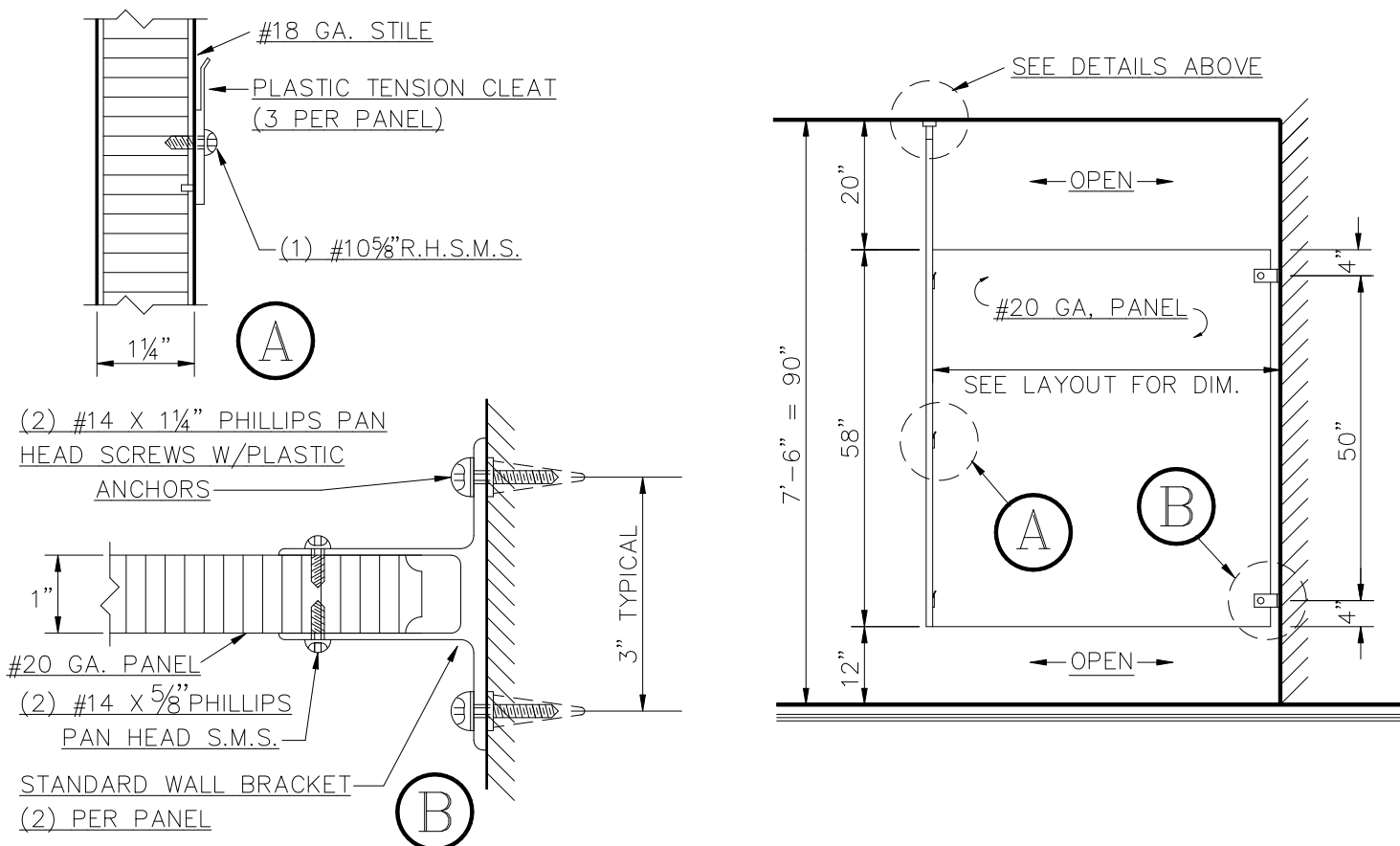
TYPE B.E. - C.S. STILE & PANEL INSTALLATION
