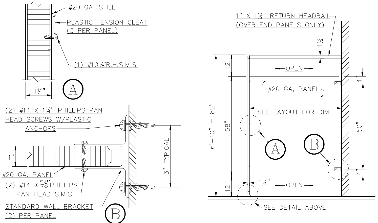
TYPE B.E.-F.F. STILE & PANEL INSTALLATION
