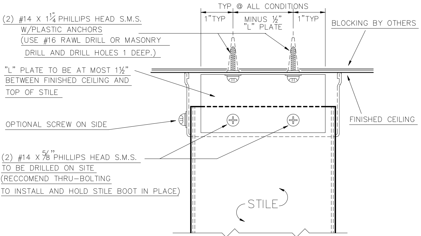
TYPE B.E. - FLR./CLG. CELING FASTENING INSTALLATION
