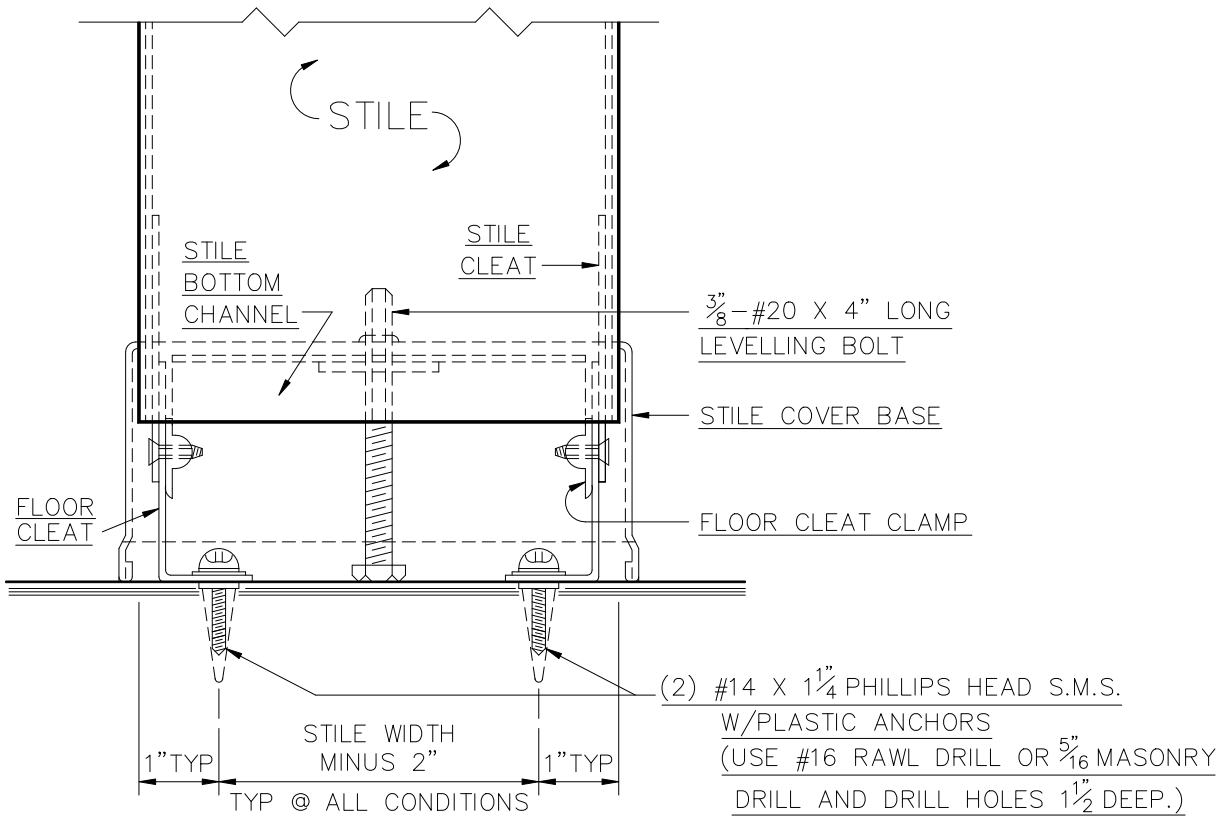
TYPE B.E. - FLR/CLG. FLOOR FASTENING ASSEMBLY
