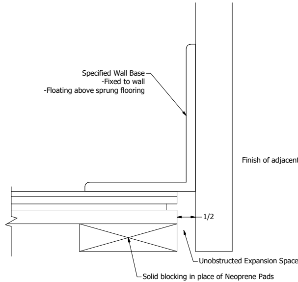
Wall Base Detail
