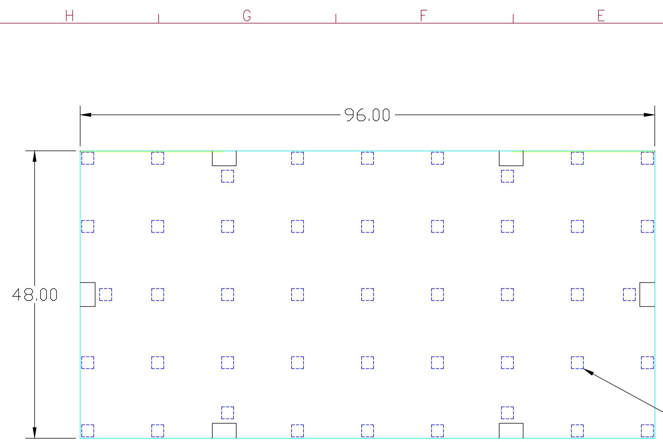
96" X 48" [2428 X 1219mm] STAGE PANEL
