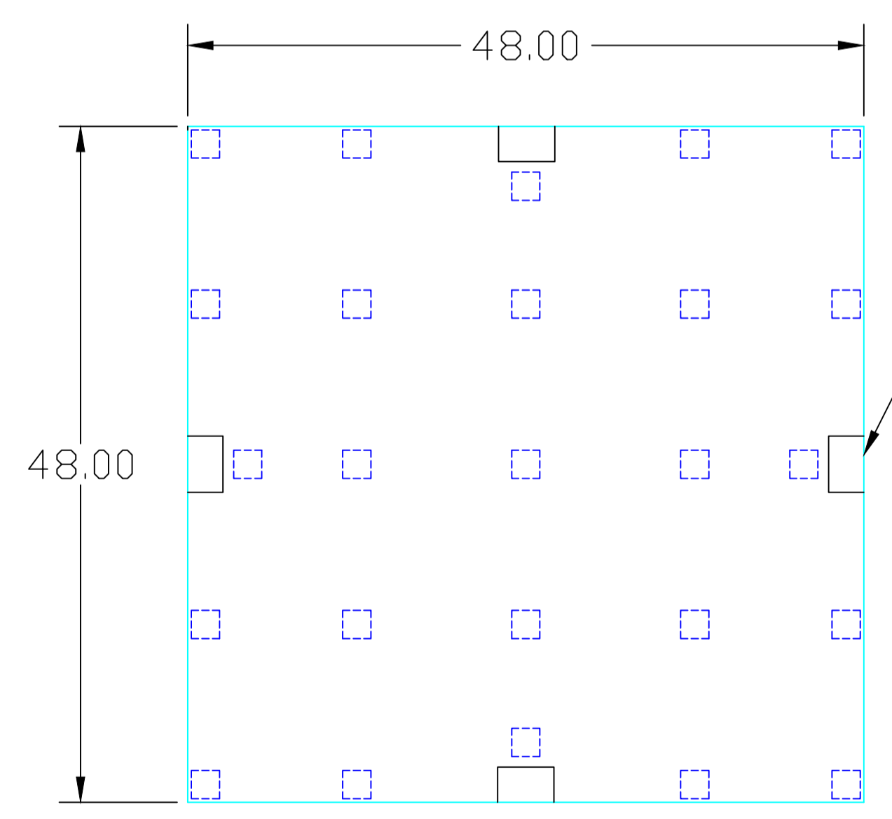
48" X 48" [1219 X 1219mm] STAGE PANEL
