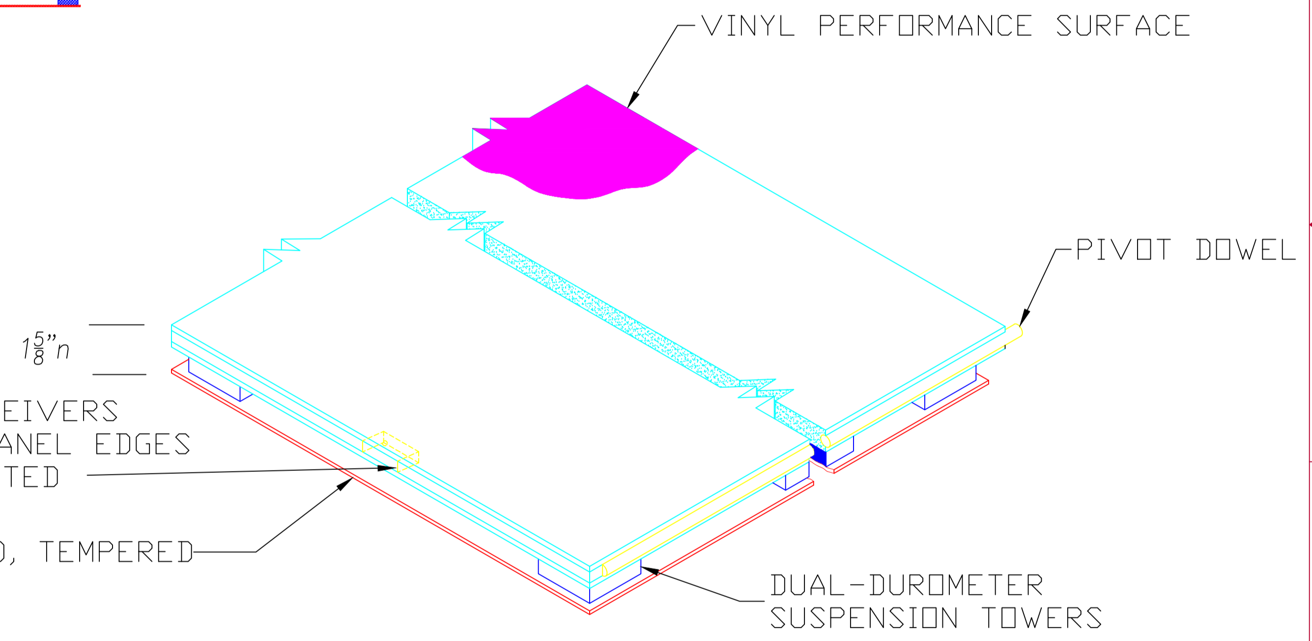
ISOMETRIC CUTAWAY VIEW OF FLOOR PANEL
