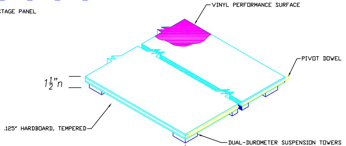
ISOMETRIC CUTAWAY VIEW OF FLOOR PANEL
