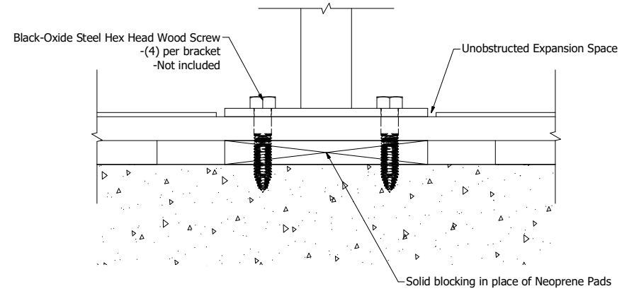
Fixing Detail
