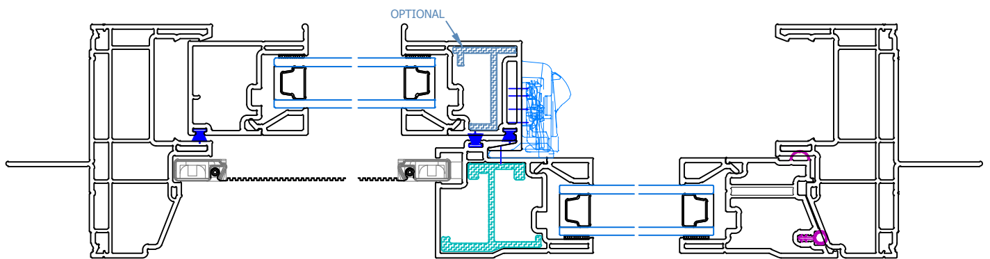
Section B-B
