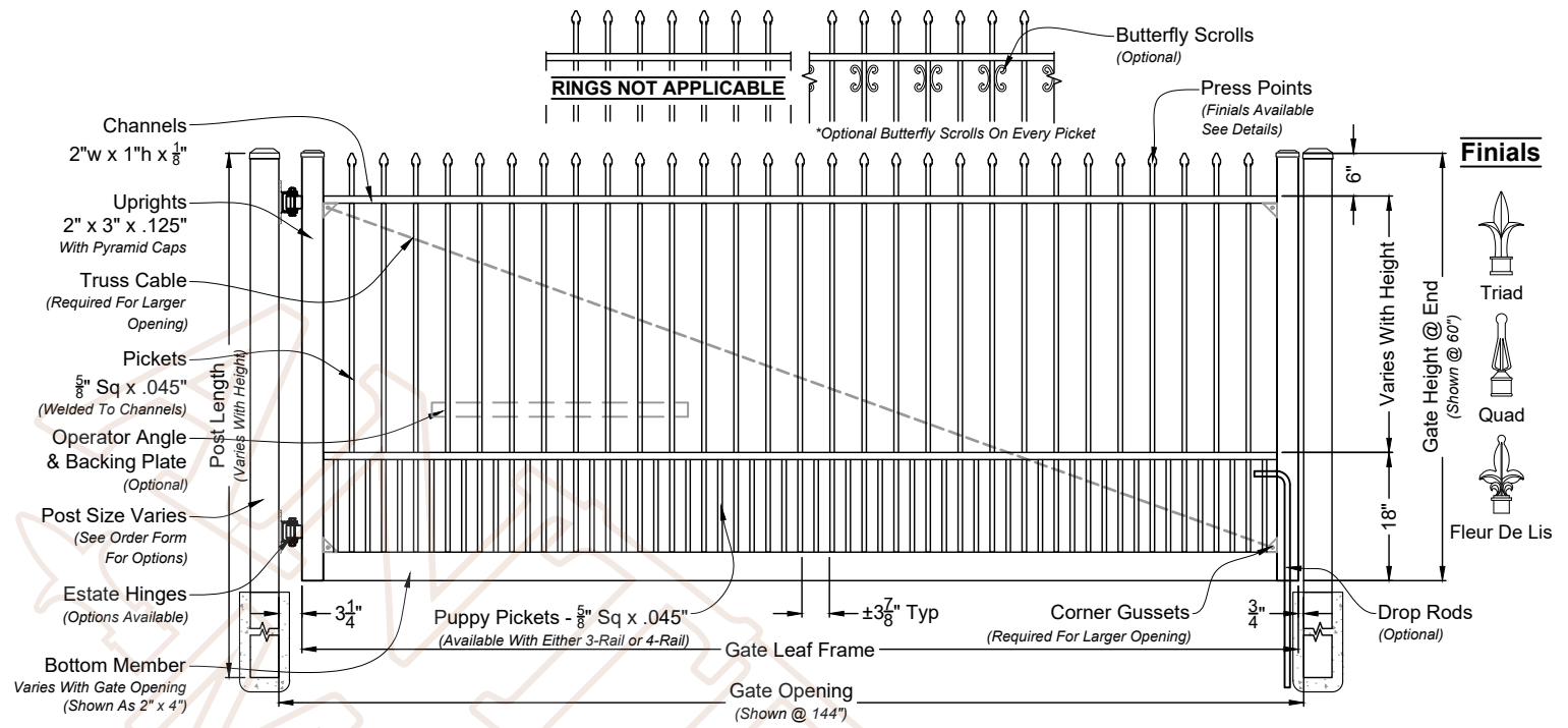
A 01 Abigail Single Estate Gate Shown As Residential Series Scale: NTS *Displayed As Standard
