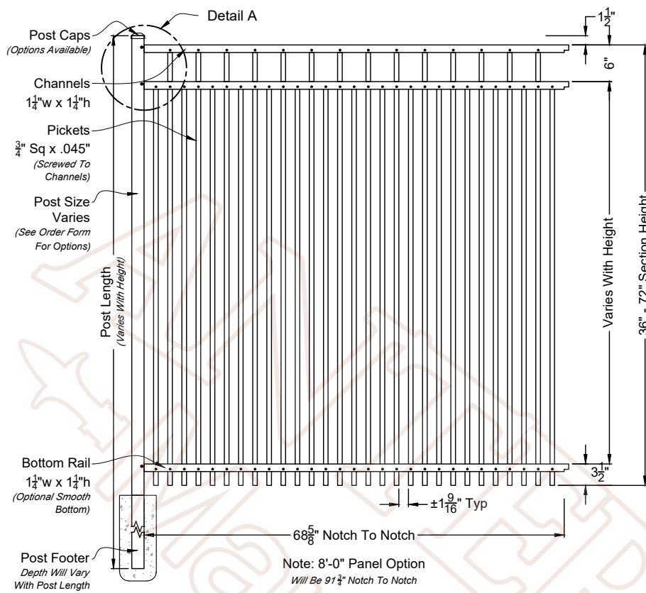
A 01 Bella Rae 6ft Wide Fence Panel Shown As Commercial Series Scale: NTS *Displayed As Rake Bottom; Also Available As Smooth Bottom
