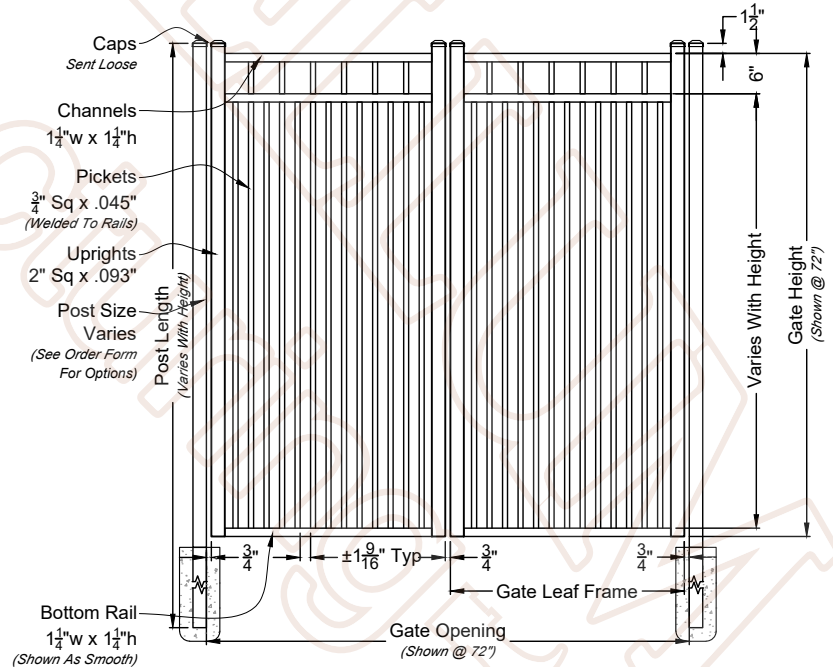
A 03 Bella Rae Double Walk Gate Shown With Straight Rail Option Scale: NTS *Displayed As Smooth Bottom; Also Available As Rake Bottom
