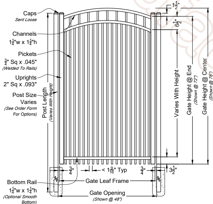
A 02 Bella Rae Single Walk Gate Shown with Arched Rail Option Scale: NTS *Displayed As Rake Bottom; Also Available As Smooth Bottom
