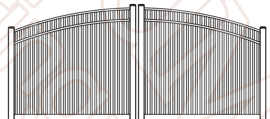
A 04 Arch Options All Considered Standard Scale: NTS *Arch Follows 1" Of Rise For Every Foot Of Opening
