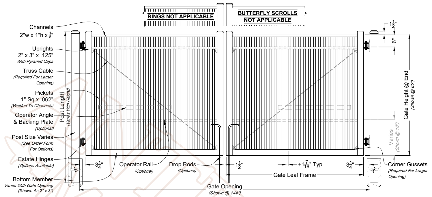
A 01 Emily Double Estate Gate Shown As Industrial Series Scale: NTS *Displayed As Standard
