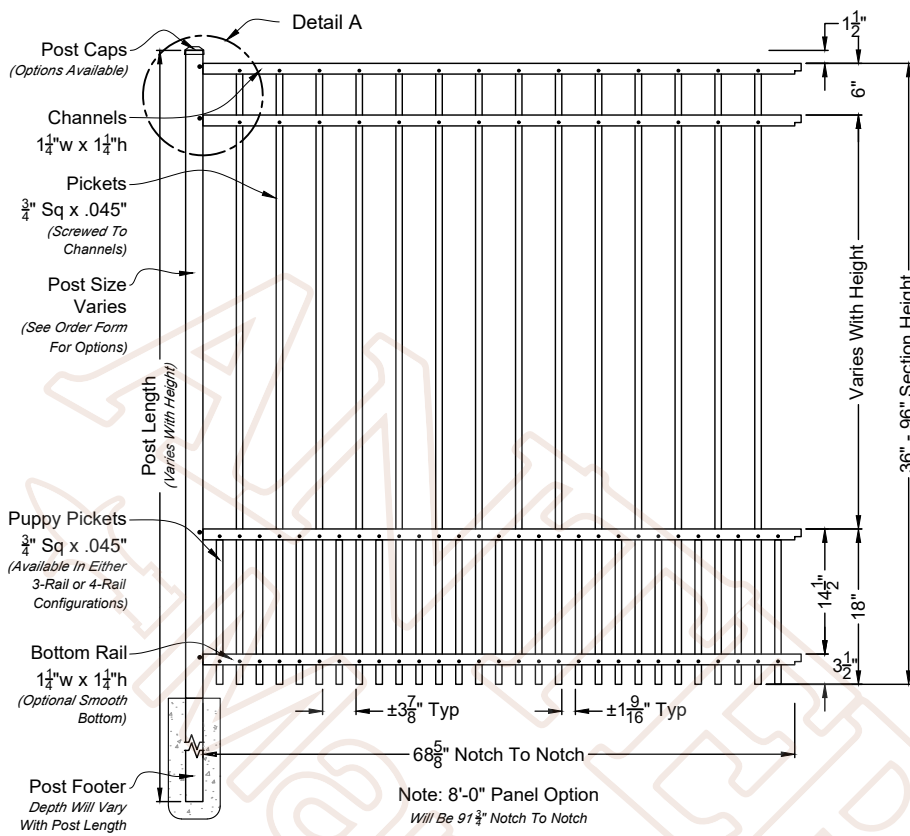
A 01 Emily 6ft Wide Fence Panel Shown As Commercial Series Scale: NTS *Displayed As Rake Bottom; Also Available As Smooth Bottom
