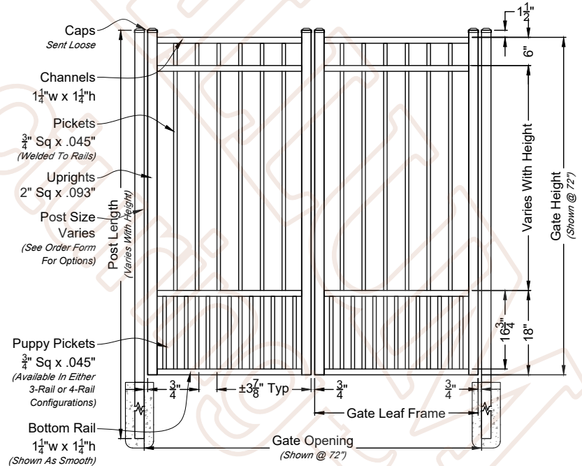
A 03 Emily Double Walk Gate Shown With Straight Rail Option Scale: NTS *Displayed As Smooth Bottom; Also Available As Rake Bottom
