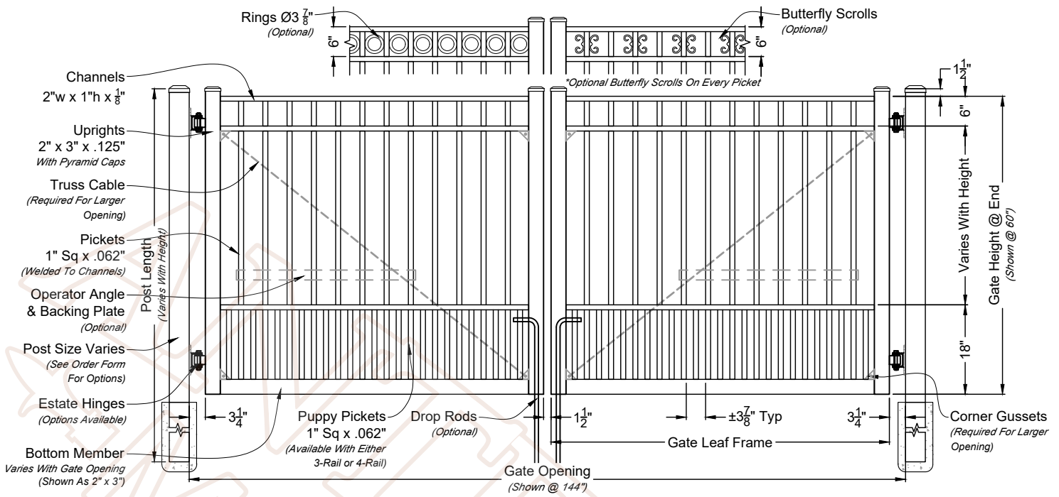
A 01 Emily Double Estate Gate Shown As Industrial Series Scale: NTS *Displayed As Standard
