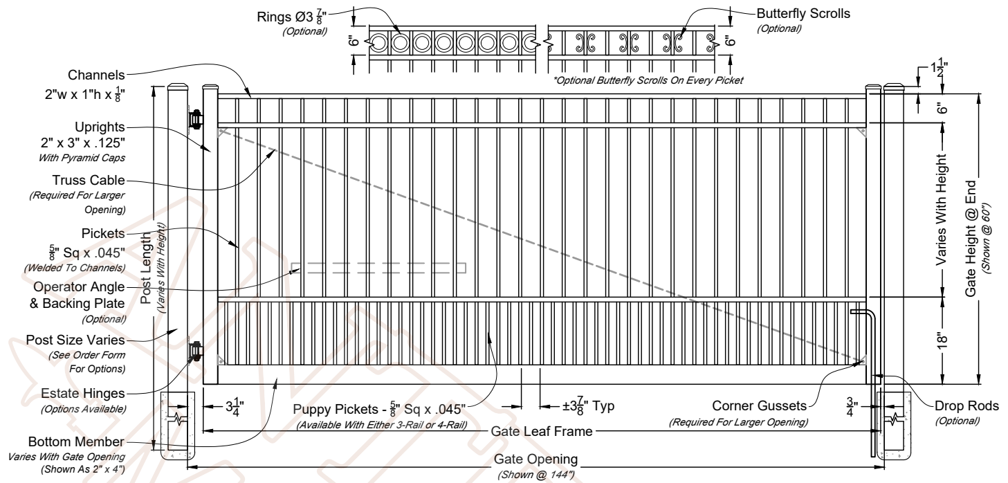
A 01 Emily Single Estate Gate Shown As Residential Series Scale: NTS *Displayed As Standard
