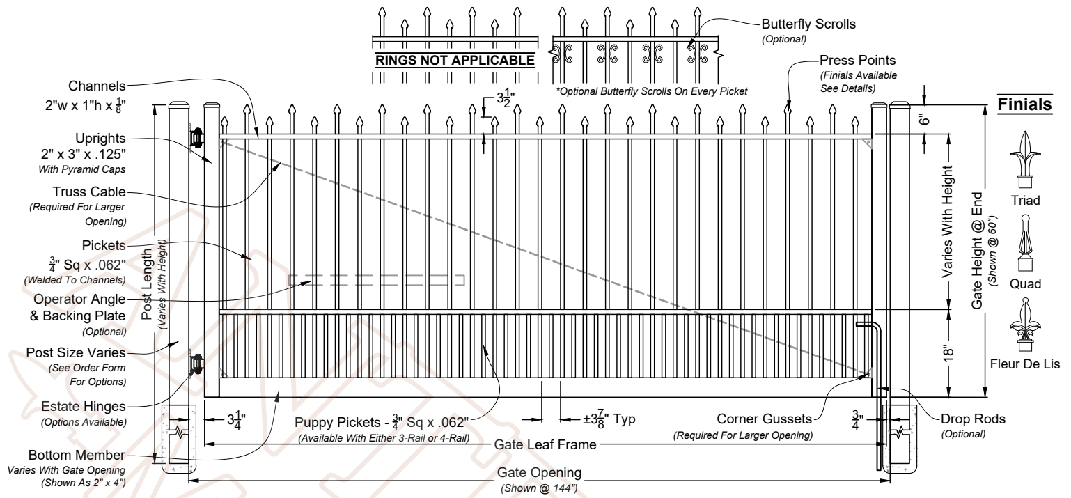
A 01 Madison Single Estate Gate Shown As Commercial Series Scale: NTS *Displayed As Standard
