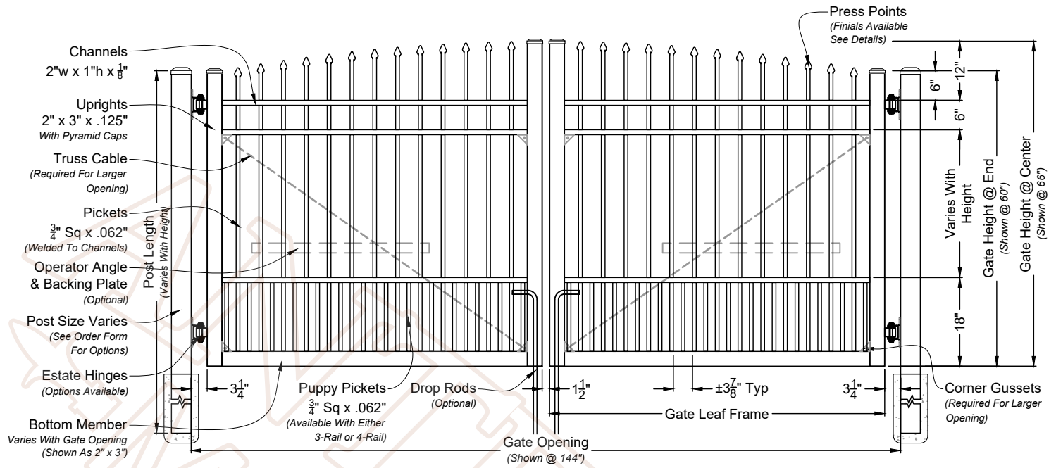
A Walker Double Estate Gate 01 Shown As Commercial Series Scale: NTS *Displayed As Standard
