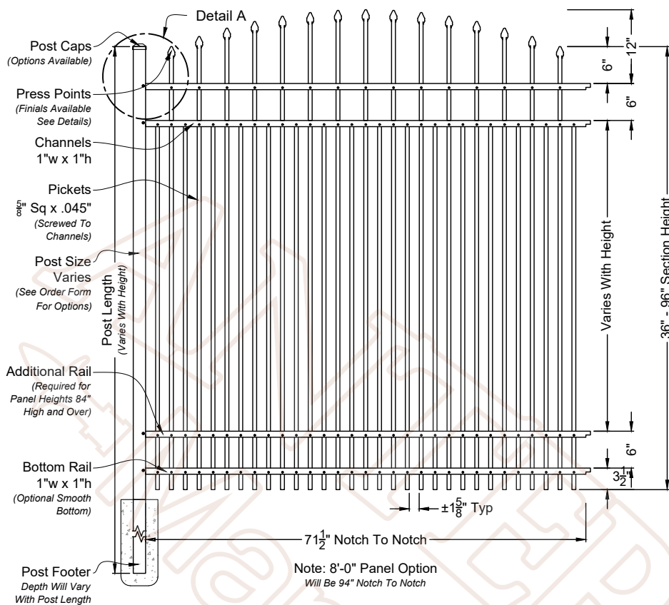
A Walker 6ft Wide Fence Panel 01 Shown As Residential Series Scale: NTS *Displayed As Rake Bottom; Also Available As Smooth Bottom
