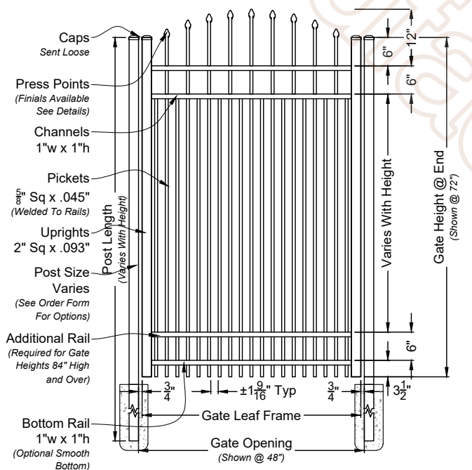
A Walker Single Walk Gate 02 Shown with Arched Rail Option Scale: NTS *Displayed As Rake Bottom; Also Available As Smooth Bottom
