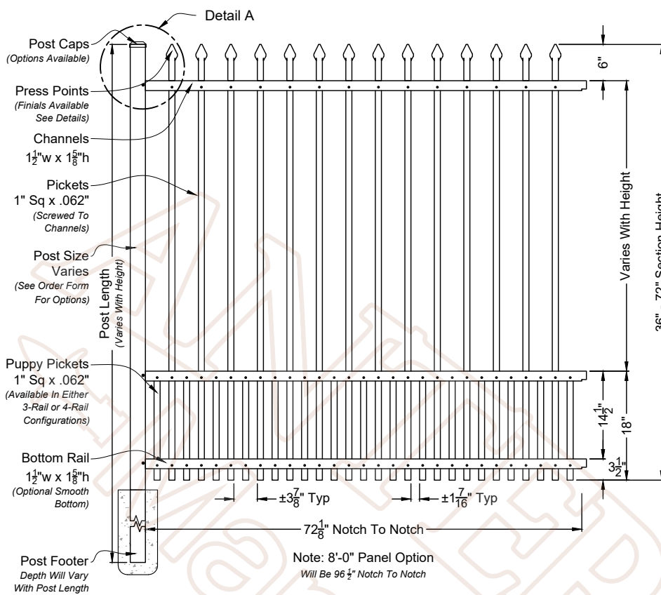
A 01 Abigail 6ft Wide Fence Panel Shown As Industrial Series Scale: NTS *Displayed As Rake Bottom; Also Available As Smooth Bottom
