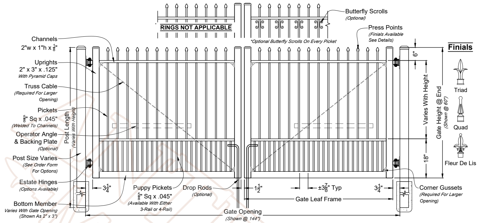
A 01 Abigail Double Estate Gate Shown As Residential Series Scale: NTS *Displayed As Standard
