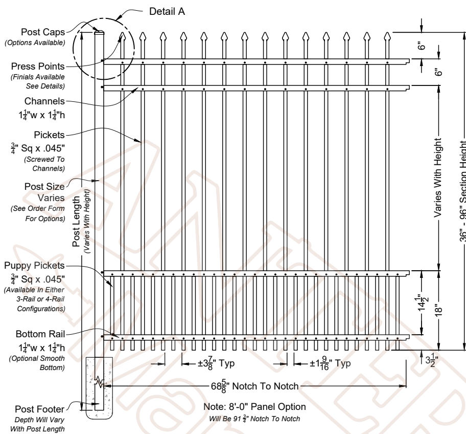
A 01 Abigail 6ft Wide Fence Panel Shown As Commercial Series Scale: NTS *Displayed As Rake Bottom; Also Available As Smooth Bottom
