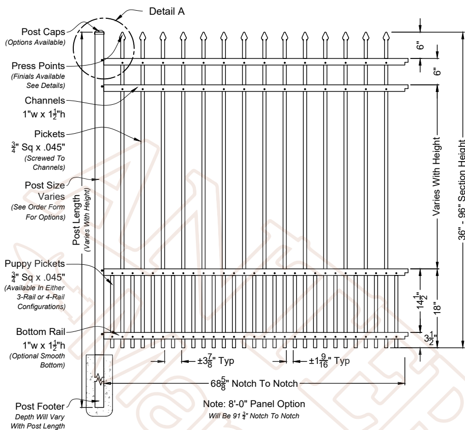
A 01 Abigail 6ft Wide Fence Panel Shown As Corporate Series Scale: NTS *Displayed As Rake Bottom; Also Available As Smooth Bottom
