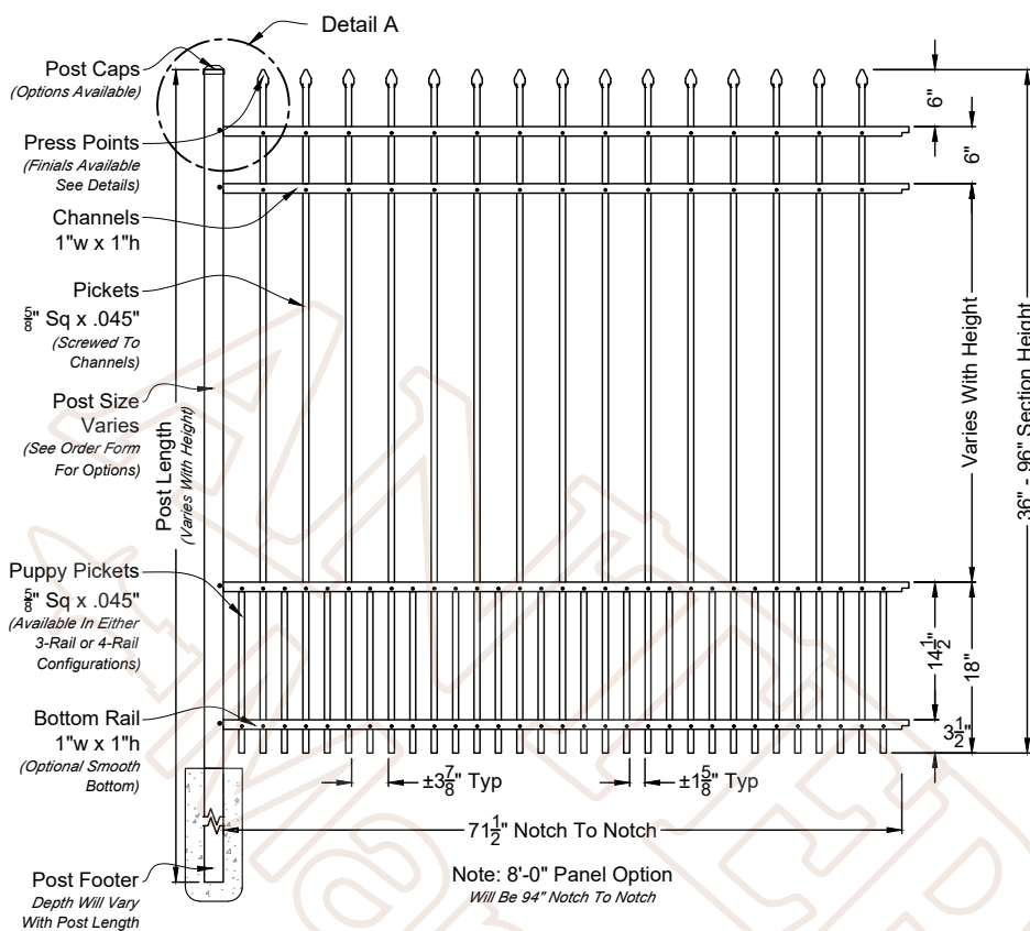
A 01 Abigail 6ft Wide Fence Panel Shown As Residential Series Scale: NTS *Displayed As Rake Bottom; Also Available As Smooth Bottom
