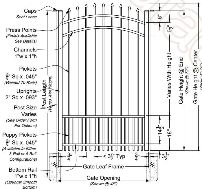
A 02 Abigail Single Walk Gate Shown with Arched Rail Option Scale: NTS *Displayed As Rake Bottom; Also Available As Smooth Bottom
