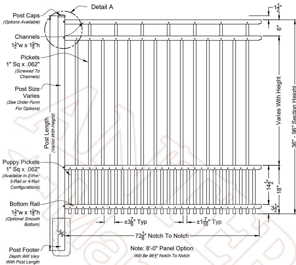
A 01 Bella Rae 6ft Wide Fence Panel Shown As Industrial Series Scale: NTS *Displayed As Rake Bottom; Also Available As Smooth Bottom
