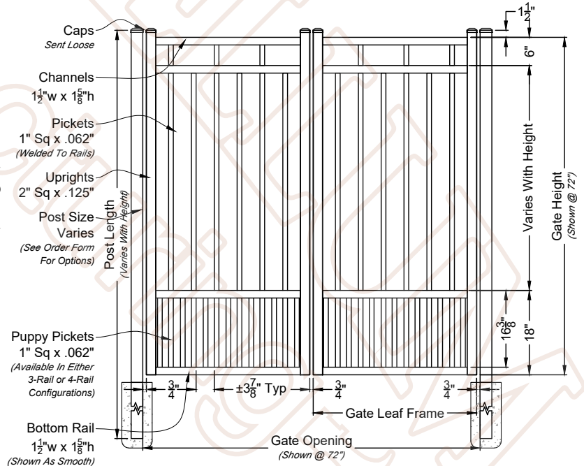
A 03 Bella Rae Double Walk Gate Shown With Straight Rail Option Scale: NTS *Displayed As Smooth Bottom; Also Available As Rake Bottom
