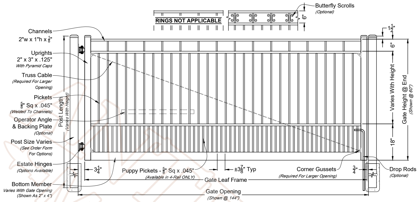
A 01 Bella Rae Single Estate Gate Shown As Residential Series Scale: NTS *Displayed As Standard
