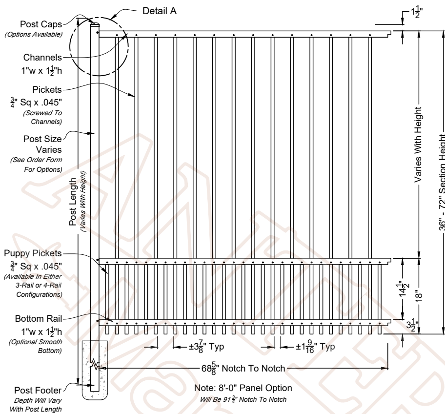
A 01 Emily 6ft Wide Fence Panel Shown As Corporate Series Scale: NTS *Displayed As Rake Bottom; Also Available As Smooth Bottom
