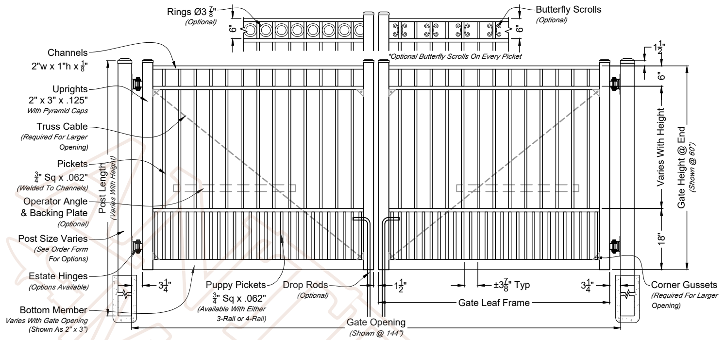
A 01 Emily Double Estate Gate Shown As Commercial Series Scale: NTS *Displayed As Standard
