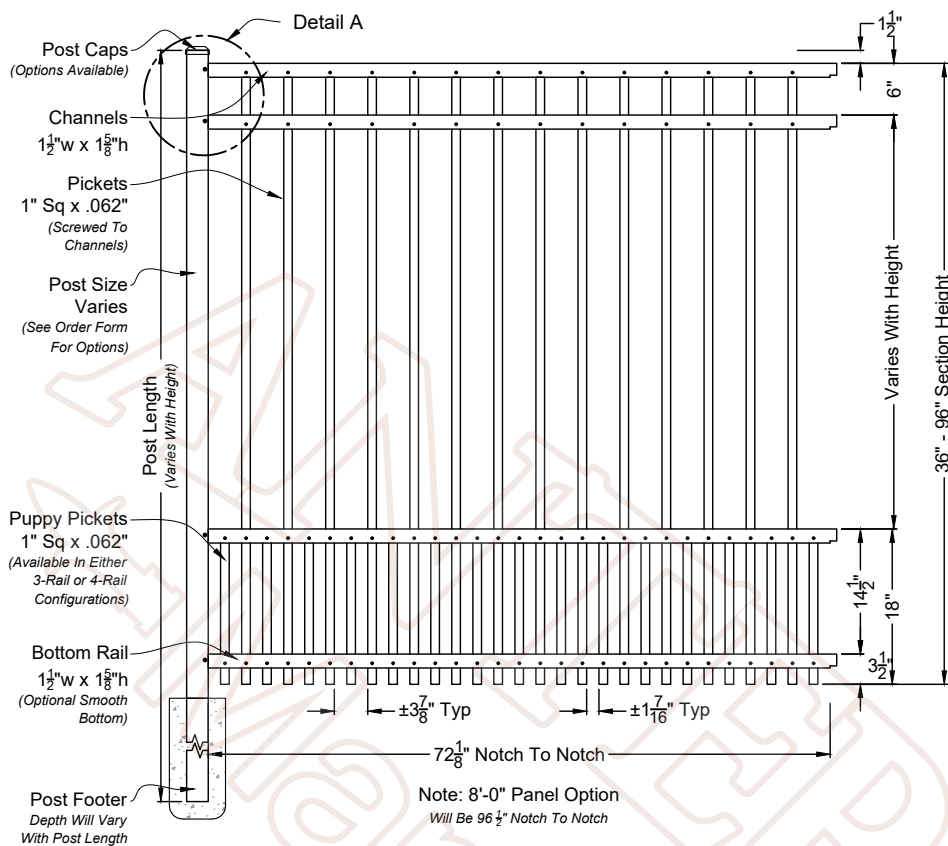
A 01 Emily 6ft Wide Fence Panel Shown As Industrial Series Scale: NTS *Displayed As Rake Bottom; Also Available As Smooth Bottom
