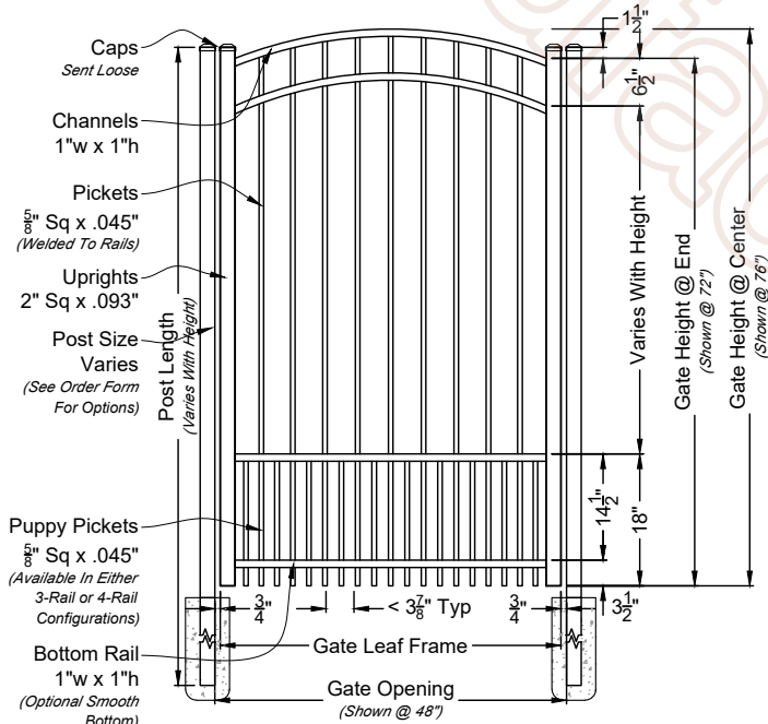
A 02 Emily Single Walk Gate Shown with Arched Rail Option Scale: NTS *Displayed As Rake Bottom; Also Available As Smooth Bottom
