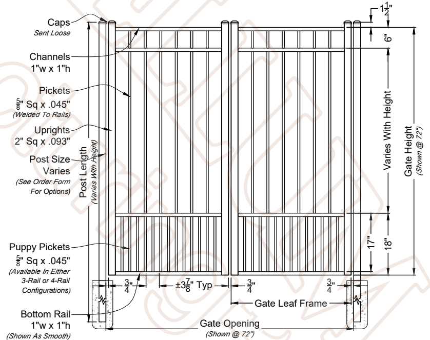
A 03 Emily Double Walk Gate Shown With Straight Rail Option Scale: NTS *Displayed As Smooth Bottom; Also Available As Rake Bottom
