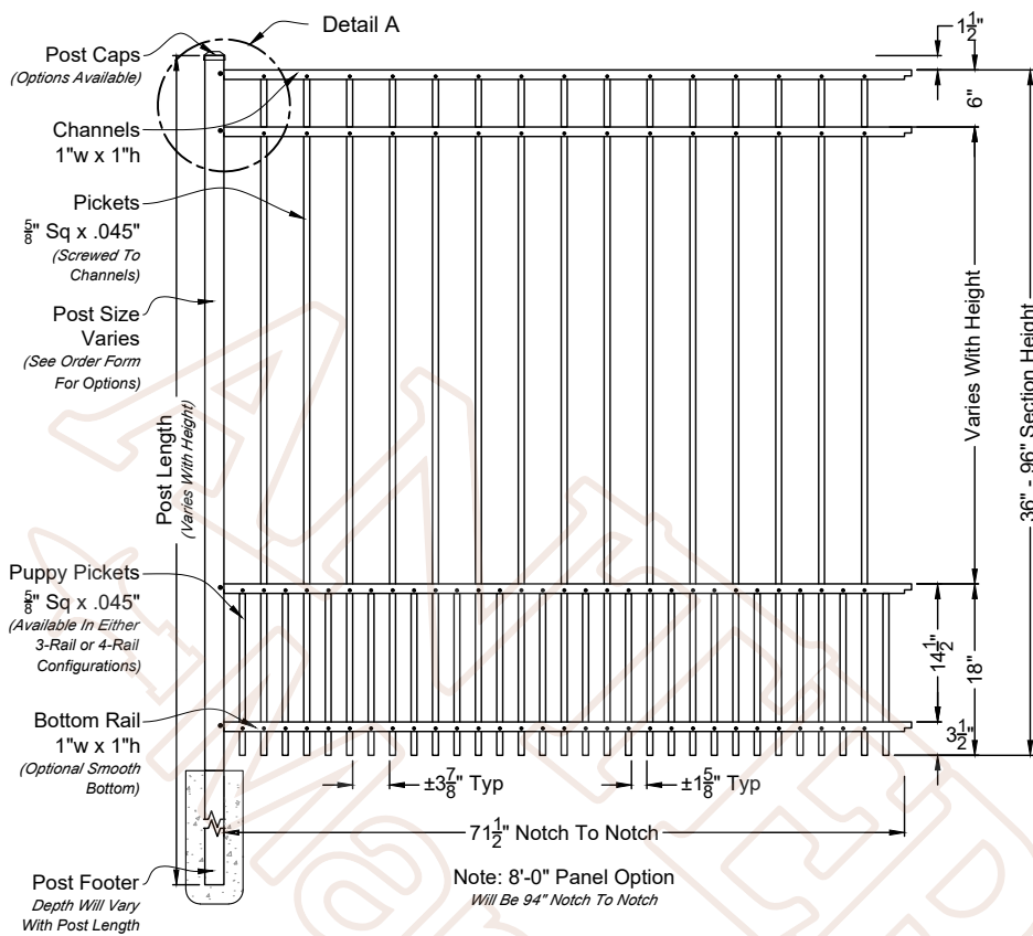
A 01 Emily 6ft Wide Fence Panel Shown As Residential Series Scale: NTS *Displayed As Rake Bottom; Also Available As Smooth Bottom
