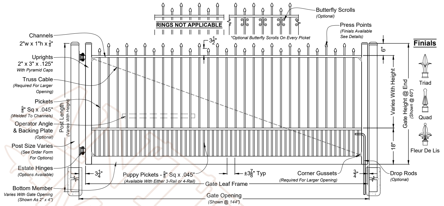
A 01 Madison Single Estate Gate Shown As Residential Series Scale: NTS *Displayed As Standard
