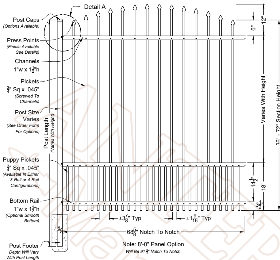
Walker 6ft Wide Fence Panel 01 Shown As Corporate Series Scale: NTS *Displayed As Rake Bottom; Also Available As Smooth Bottom
