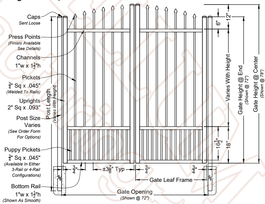
Walker Double Walk Gate 03 Shown With Straight Rail Option Scale: NTS *Displayed As Smooth Bottom; Also Available As Rake Bottom
