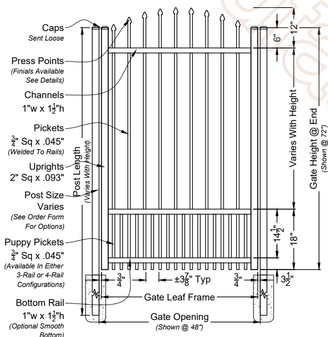
Walker Single Walk Gate 02 Shown with Arched Rail Option Scale: NTS *Displayed As Rake Bottom; Also Available As Smooth Bottom
