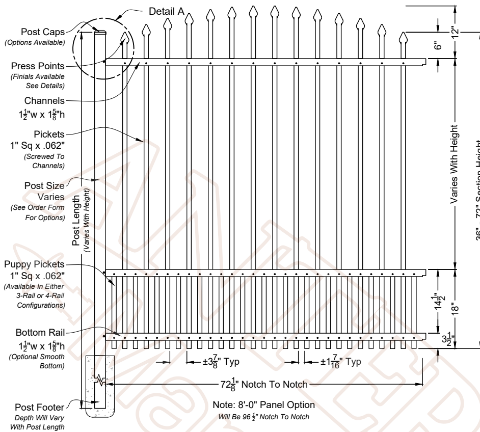
A 01 Walker 6ft Wide Fence Panel Shown As Industrial Series Scale: NTS *Displayed As Rake Bottom; Also Available As Smooth Bottom
