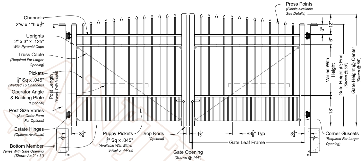
A Walker Double Estate Gate 01 Shown As Residential Series Scale: NTS *Displayed As Standard
