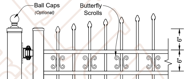
A Butterfly Scrolls 05 Shown Every Other Picket Scale: NTS *Optional Butterfly Scrolls On Every Picket
