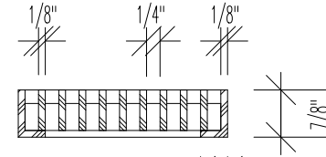
SECTION
