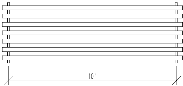
PLAN: AG20 GRILLE MODEL (Core only)
