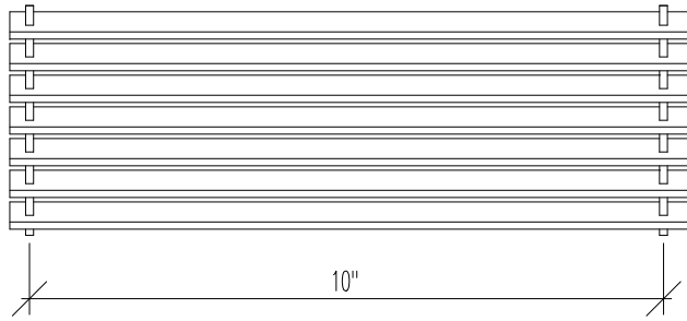
PLAN: AG40 GRILLE MODEL (Core only)
