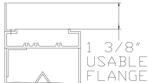
FLANGE FRAME DETAIL
