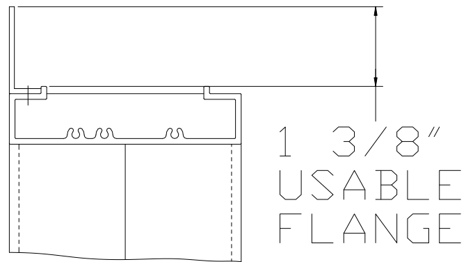
FLANGE FRAME DETAIL
