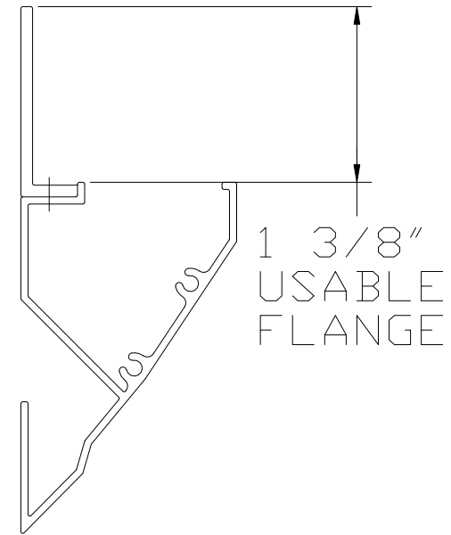
FLANGE FRAME DETAIL
